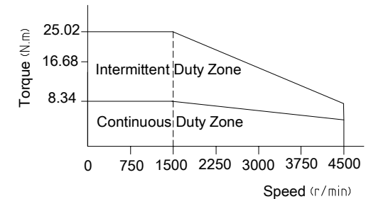
The curve of torque-speed
